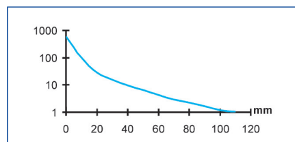
Excess gain - through beam *
