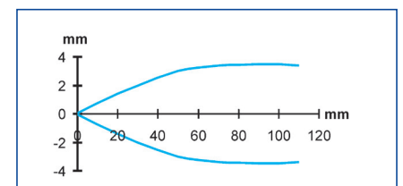
Detection area - through beam *
