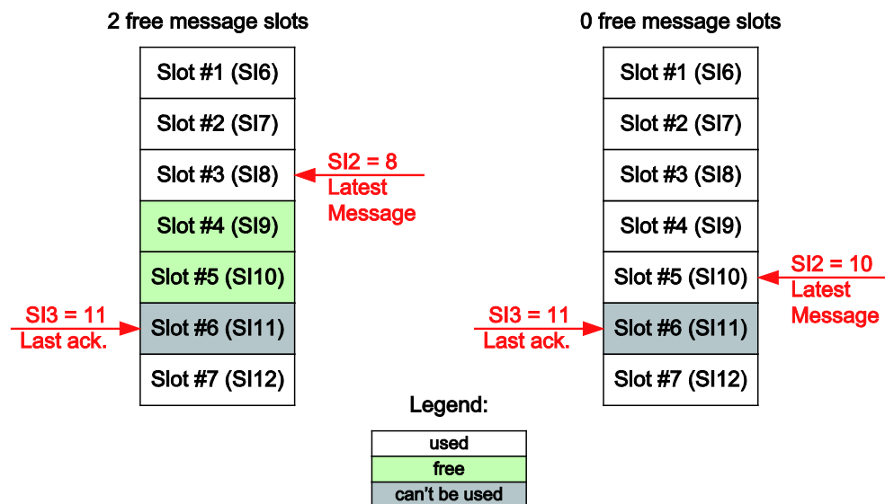
Figure 35: Number of free slots
