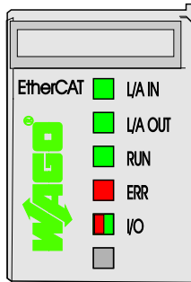
Figure 23: Display Elements
