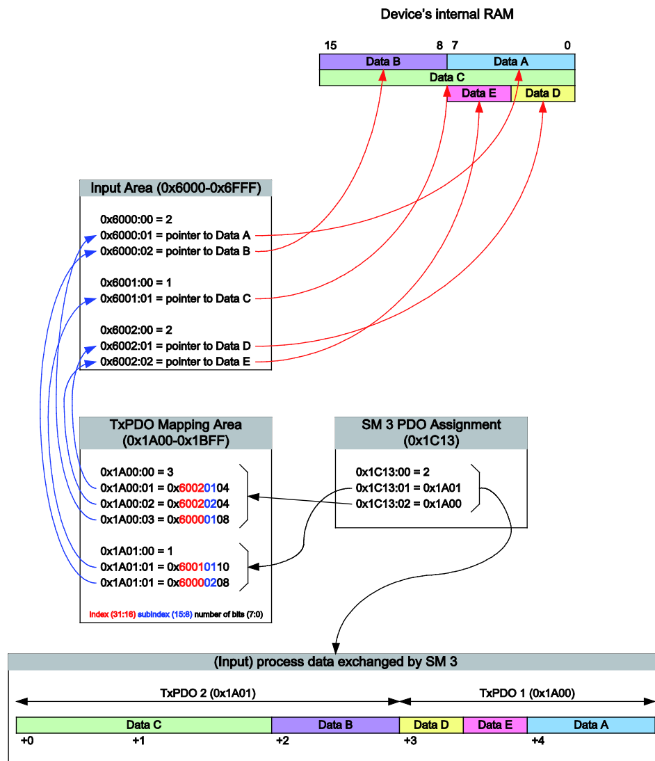
Figure 34: Example of the principle mapping of process data using EtherCAT®
