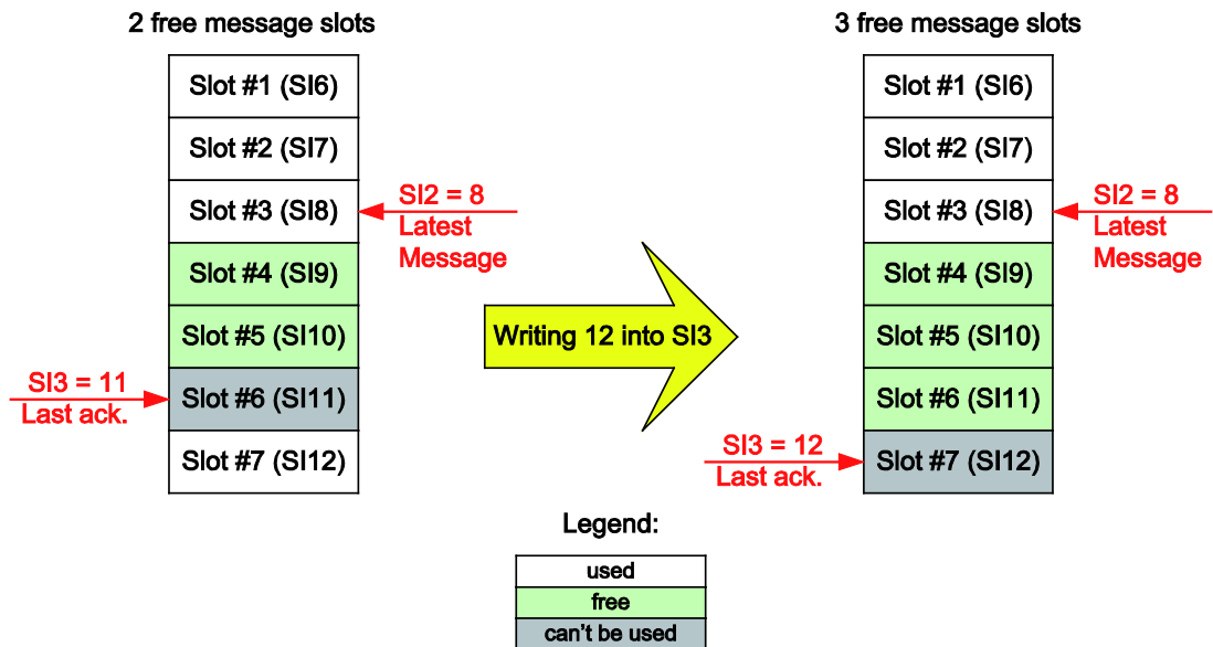
Figure 36: Acknowledgement of a diagnostic message
