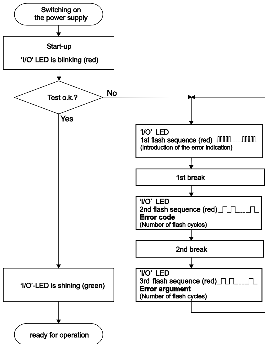
Figure 40: Node Status – I/O LED Signaling
