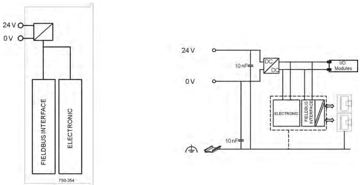
Figure 21: Device Supply
