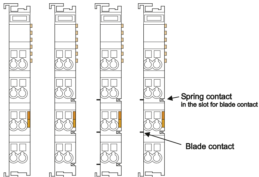
Figure 31: Example for the Arrangement of Power Contacts
