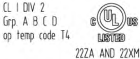
Figure 50: Text Detail – Marking Example for Approved I/O Modules According to NEC 500
