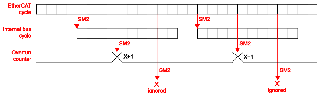
Figure 37: Overrun counter in subindex 11
