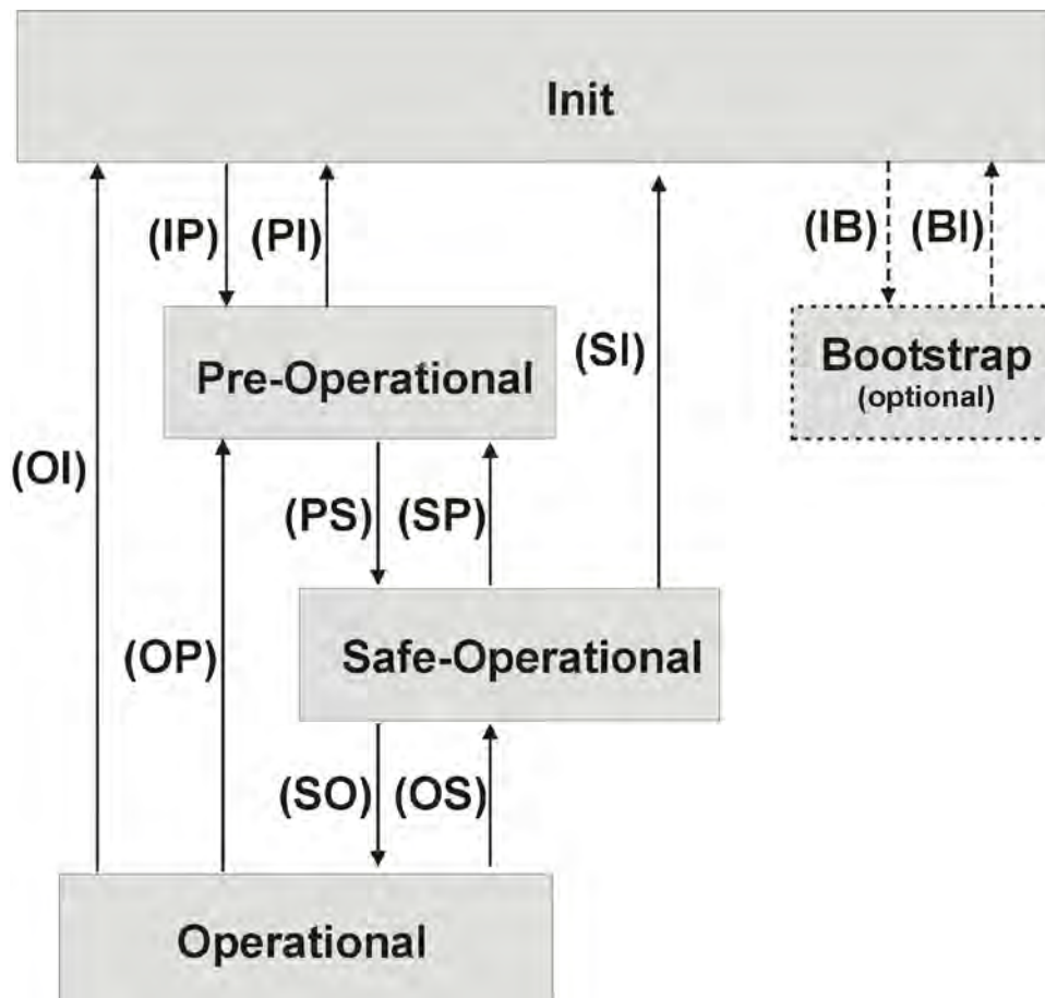
Figure 44: Status diagram of an EtherCAT® slave
