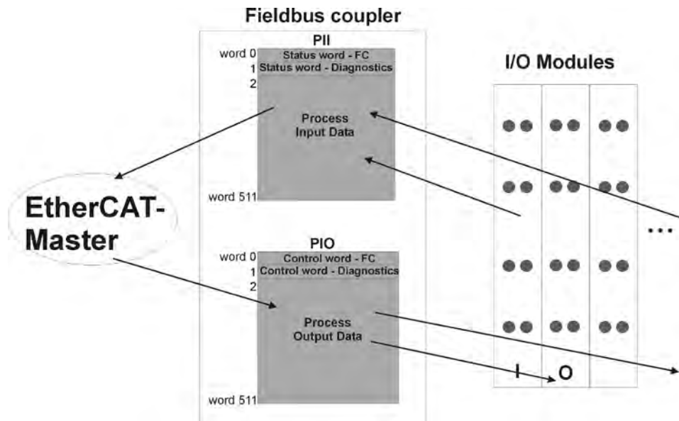
Figure 38: Memory areas and data exchange of the fieldbus coupler.
