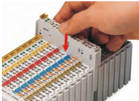
Figure 28: Snap the I/O Module into Place (Example)
