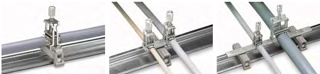
Figure 18: Examples of the WAGO Shield Connecting System
