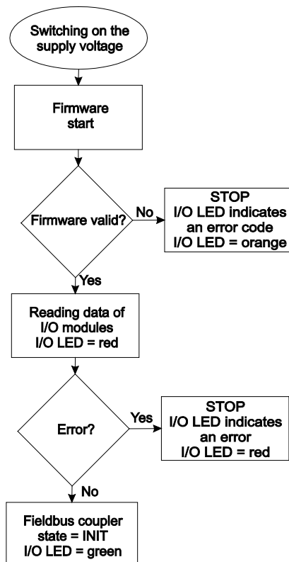
Figure 1: Starting up of the fieldbus coupler
