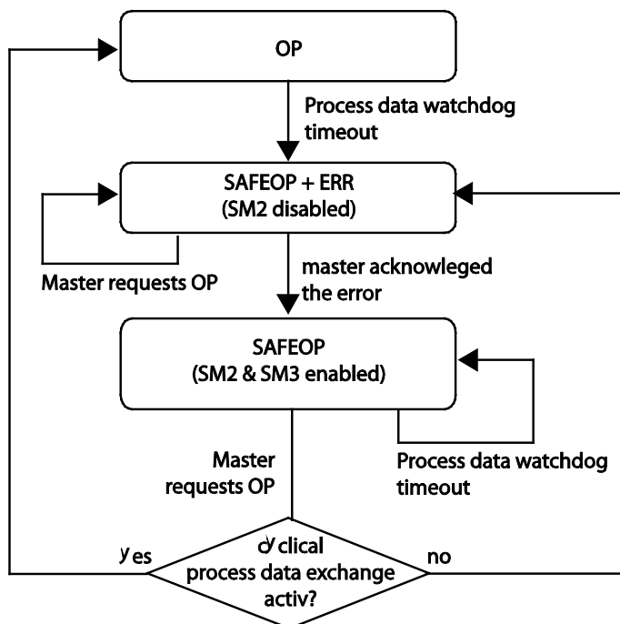
Figure 43: Error behavior of the process data watchdog
