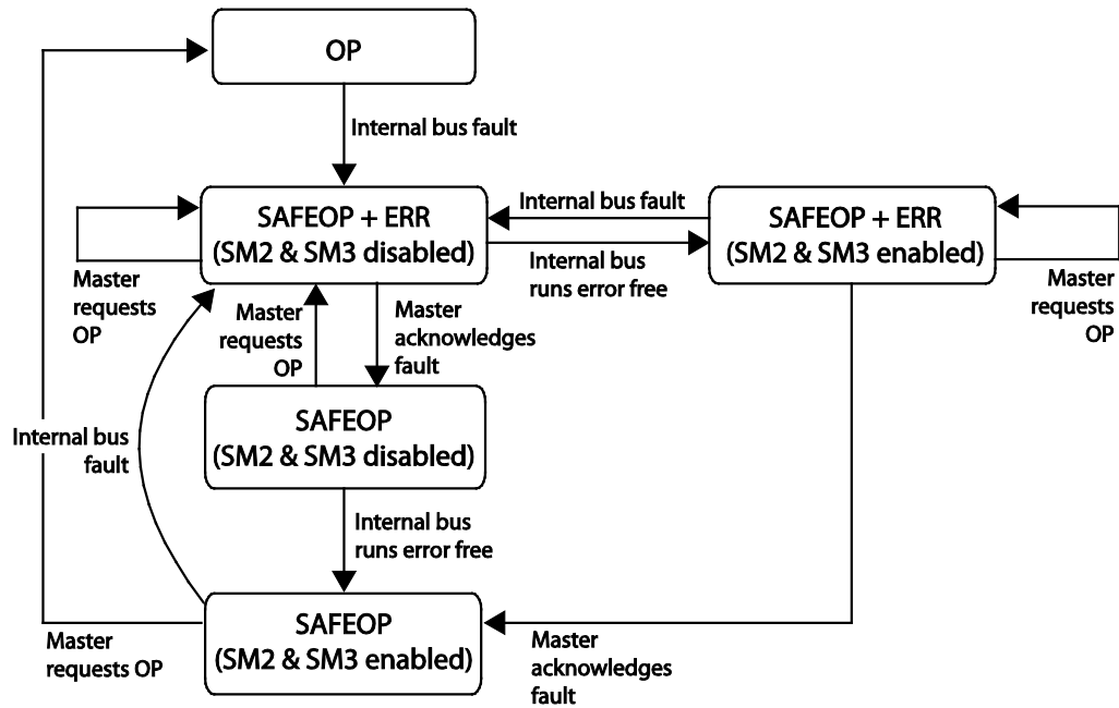
Figure 42: Behavior during an internal data bus error
