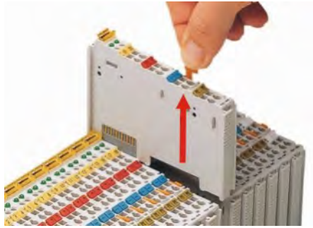
Figure 29: Removing the I/O Module (Example)
