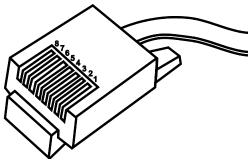
Figure 22: RJ-45 Connector
