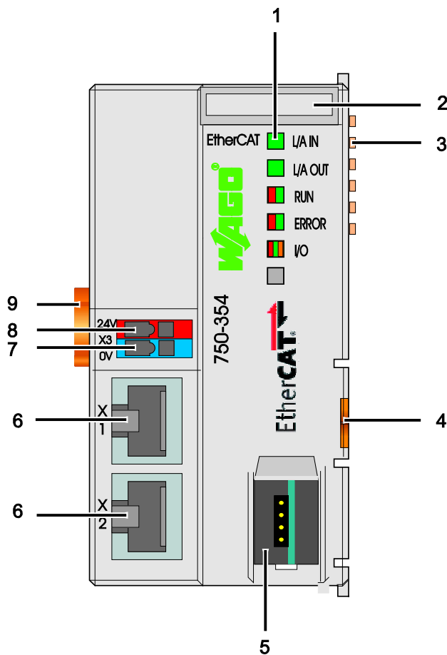
Figure 20: View EtherCAT® Fieldbus Coupler
