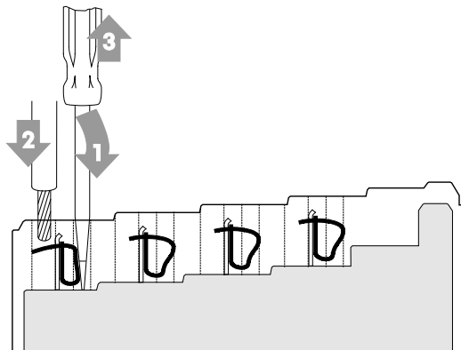
Figure 32: Connecting a Conductor to a CAGE CLAMP®
