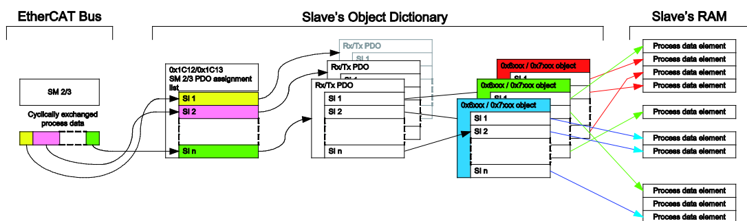
Figure 33: Mapping the Process Data
