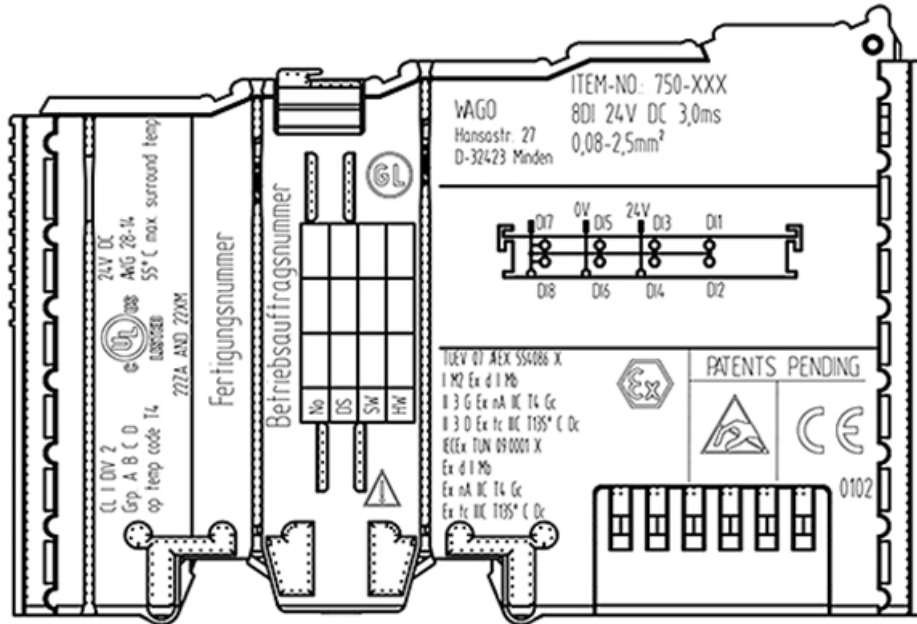
Figure 45: Side Marking Example for Approved I/O Modules According to ATEX and IECEx
