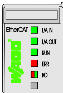
Figure 39: Display Elements
