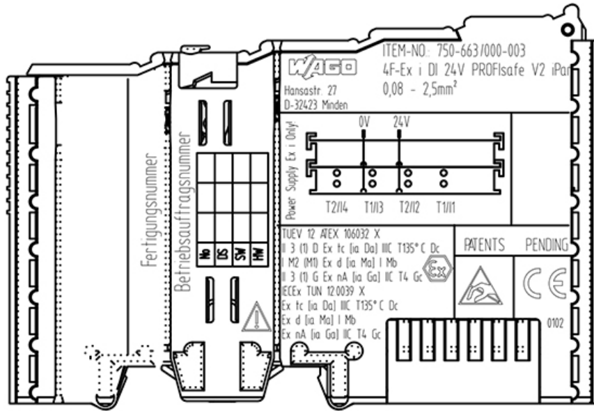
Figure 47: Side Marking Example for Approved Ex i I/O Modules According to ATEX and IECEx.
