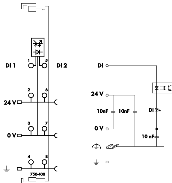
Figure 6: Schematic diagram
