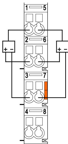
Figure 12: Connecting Diagram, 3-Conductor Connection
