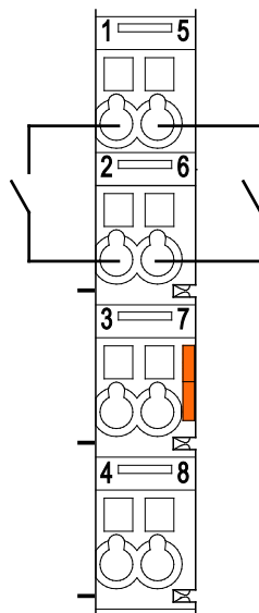
Figure 11: Connecting Diagram, 2-Conductor Connection
