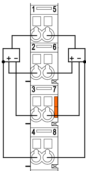
Figure 13: Connecting Diagram, 4-Conductor Connection
