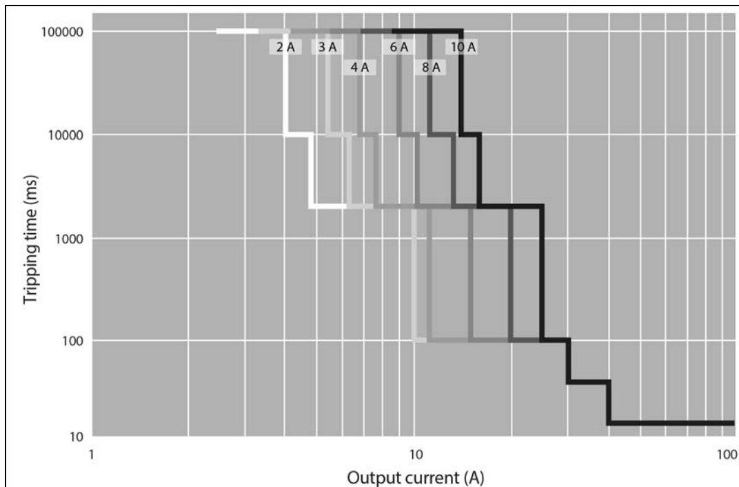
Figure 14: Trip Curve for the 10 A Circuit Breaker 787-1664
